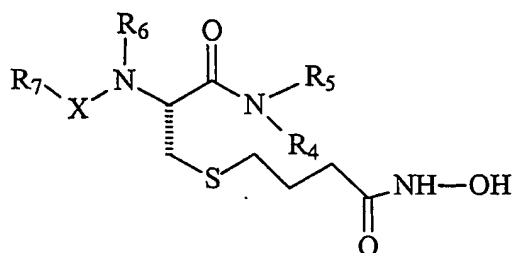
(IIIa)
